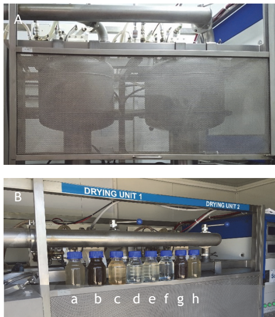
Figure 4.24 A) an experimental microwave-based faecal sludge drying unit, and B) samples taken at different points in the process: a) filtrate from the sludge press, b) concentrated sludge from the sludge press, c) ultrafiltration concentrate, d) ultrafiltration permeate, e) reverse osmosis concentrate, f) reverse osmosis permeate, g) dry sludge, and h) condensate (photo: IHE Delft).
