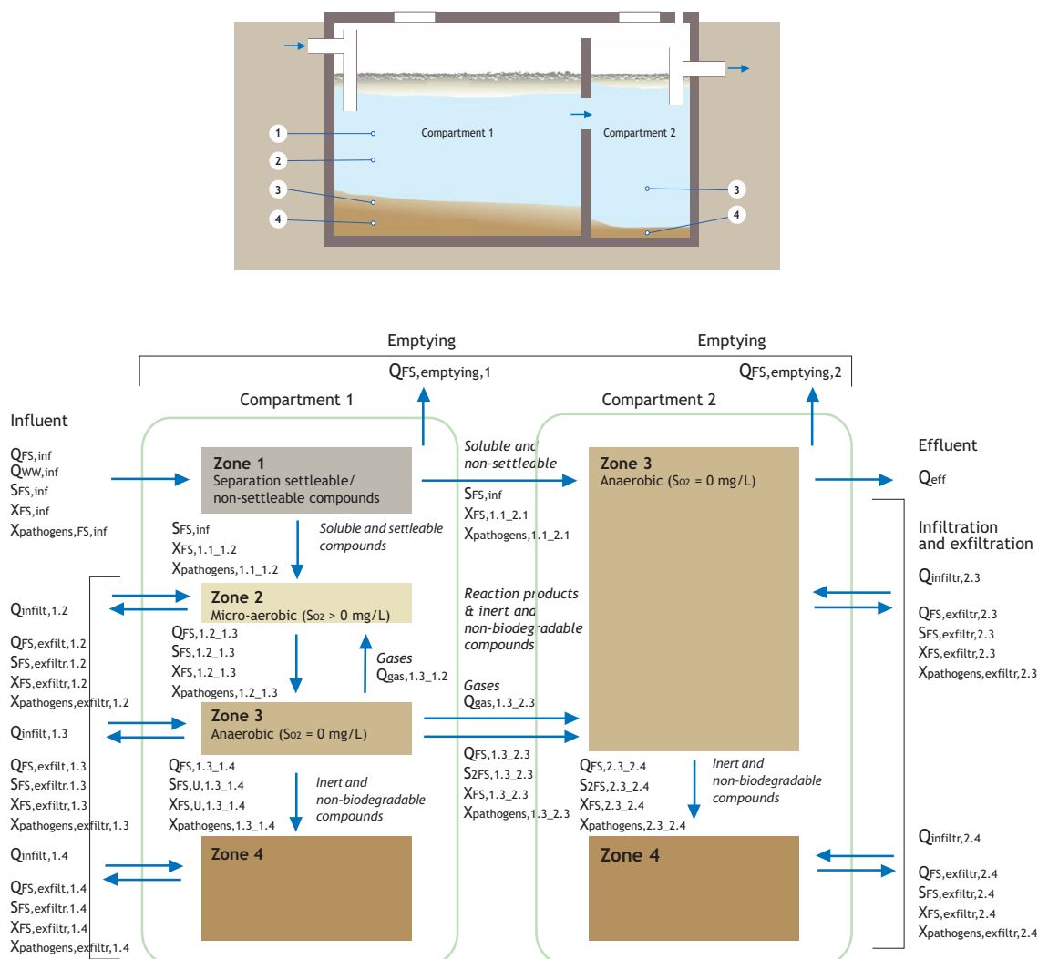
Figure 6.9 Septic tank: suggested model structure.
