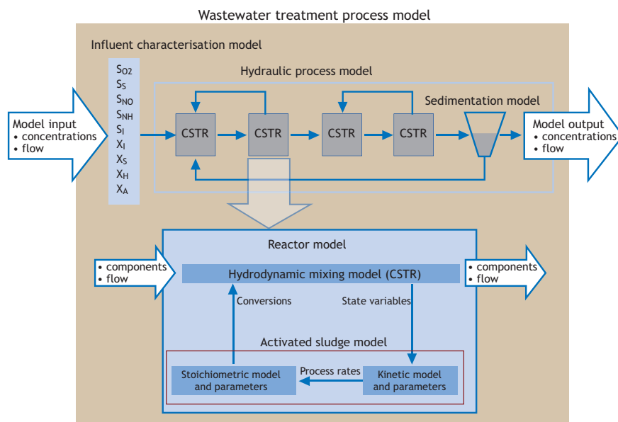
Figure 6.1 Schematic representation of an activated sludge wastewater treatment plant (modified from Meijer, 2004).
