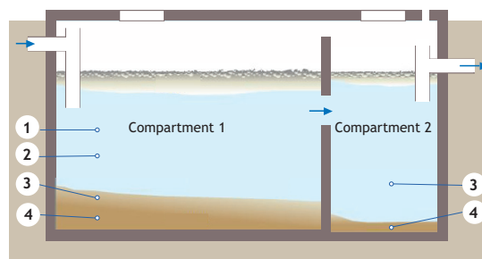
Figure 6.6 Schematic diagram illustrating the different theoretical layers within a septic tank (adapted from Tilley et al. , 2014).
