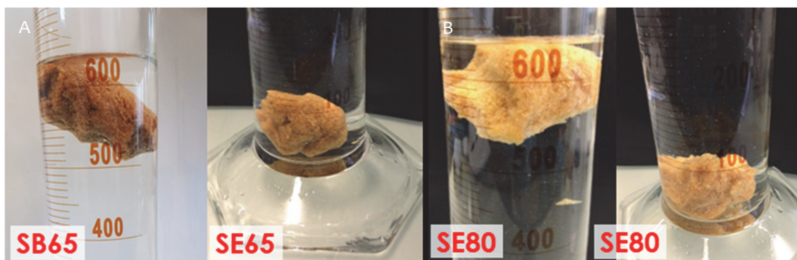
Figure 7.4 Density tests for synthetic faeces (A) S65 and (B) S80.
