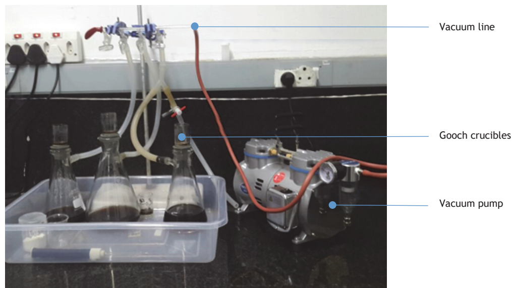
Figure 8.6 Vacuum filtration setup (photo: UKZN PRG).
