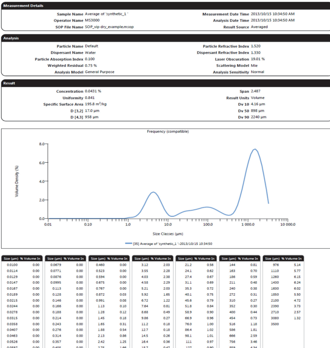
Figure 8.14 Example of data generated during the particle size analysis (source: unpublished data, UKZN PRG).
