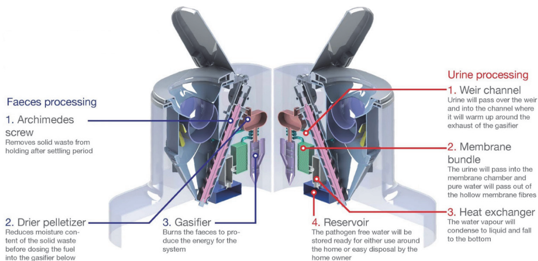
Figure 2.5 Nano Membrane toilet: an example of a waterless self-contained toilet (source: Cranfield University 3 ).
